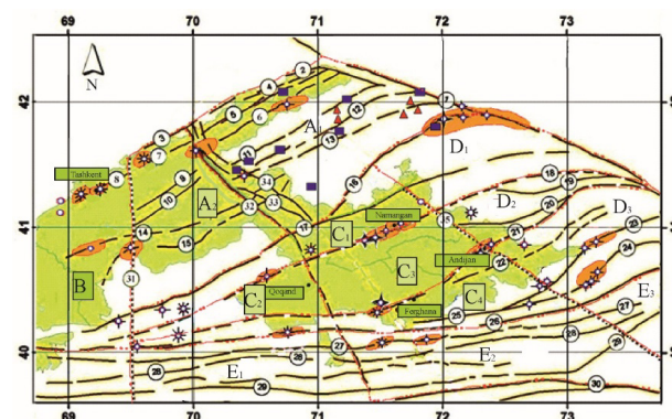
Figure 4. Highlighted 3rd-rank fault-block structures, active faults, macroseismic epicenters of strong earthquakes, and paleoseismodislocations: Active faults of the Earth's crust; Flexural-rupture zones(FRZ); - Fault-fold-block structures of the 3rd rank; - Earthquake epicenters and ; 5 – intensity of earthquakes(in points) ; 6- Paleoseismodislocations: -Researched; - Identified using satellite imagery. Active faults:1- Talas-Fergana; 2- Aksu-Maidantal; 3- Bogonali; 4- North Ugam; 5- Ugam-Maidantal; 6- Pskem; 7- Karzhantau; 8- Pre-Tashkent Flexural-Rupture Zone; 9- Syuren-Atinsky; 10- Sukok; 11- South Pskem; 12- Sandalash; 13- Chatkal; 14- North Angren; 15- South Angren; 16- Chatkal-Atoynok; 17- North Fergana; 18- North Fergana FRZ; 19- Baubashain; 20- Kuchkarota; 21- South Fergana FRZ; 22- Kugart; 23- Taldysu; 24- Kurshab; 25- Karachaty; 26- South Fergana; 27- Nuratau-Katran; 28- Karatau-Zeravshan; 29 - Main Gissar; 30 - Gissar-Kokshaal; 31- Pre-Chatkal-Kuramin; 32- Kumbel-Kokand-Haydarkan; 33- Kenkol; 34- Arashan; 35- East Fergana FRZ
